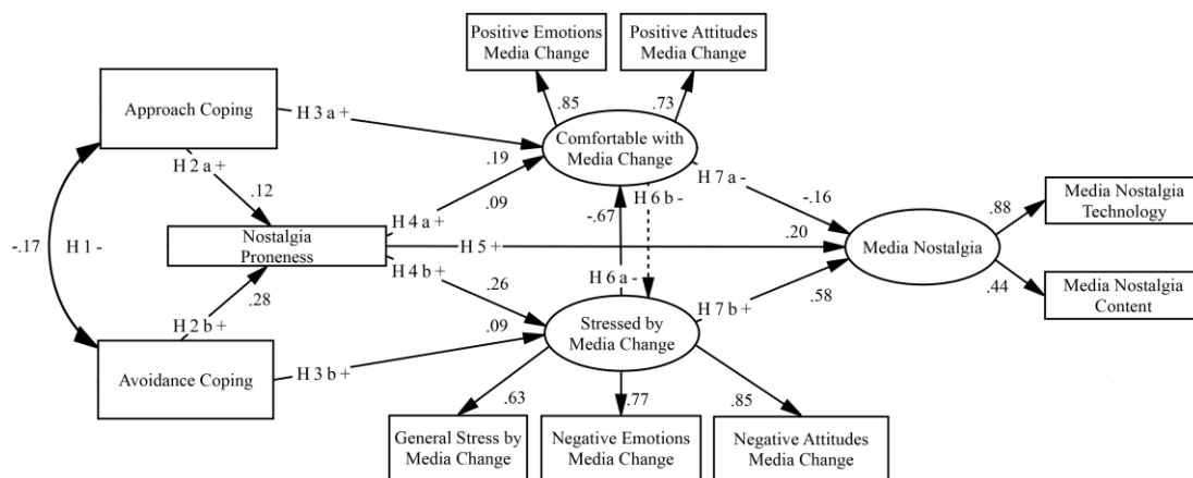
Figure 1. Observed structural equation model with hypotheses labeled.
